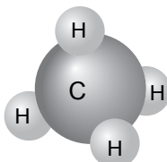
d) Methane
