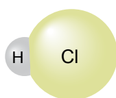
a) Hydrogen chloride
