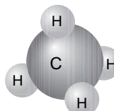
c) Methane
