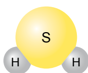
b) Hydrogen sulfide
